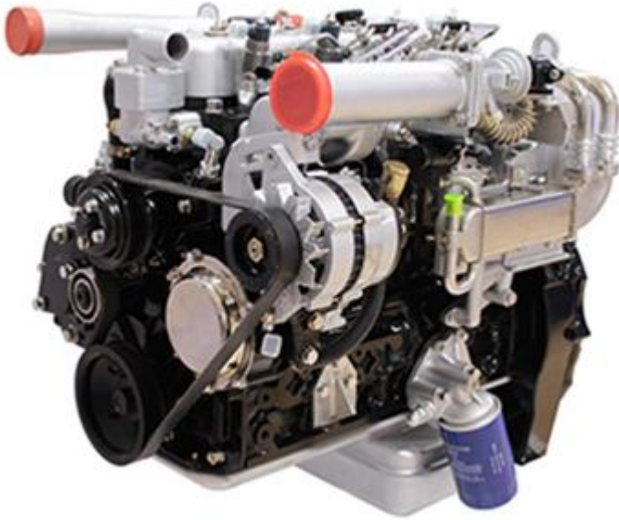
YN 4 cylinders Comply with 140hp (105Kw) at 2800 rpm Maximum input torque:550Nm
