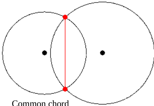
Common chord
